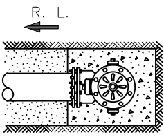
PLAN POUR CONCRETE PAD AFTER HYDRANT HAS BEEN PLACED
